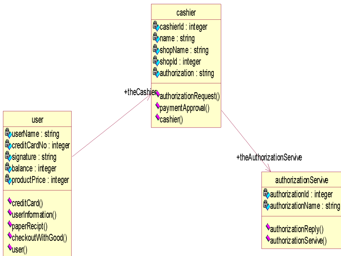
Fig.4.CLASS DIAGRAM
