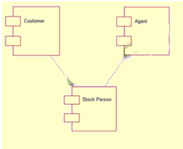
Fig.8.2.COMPONENT DIAGRAM
