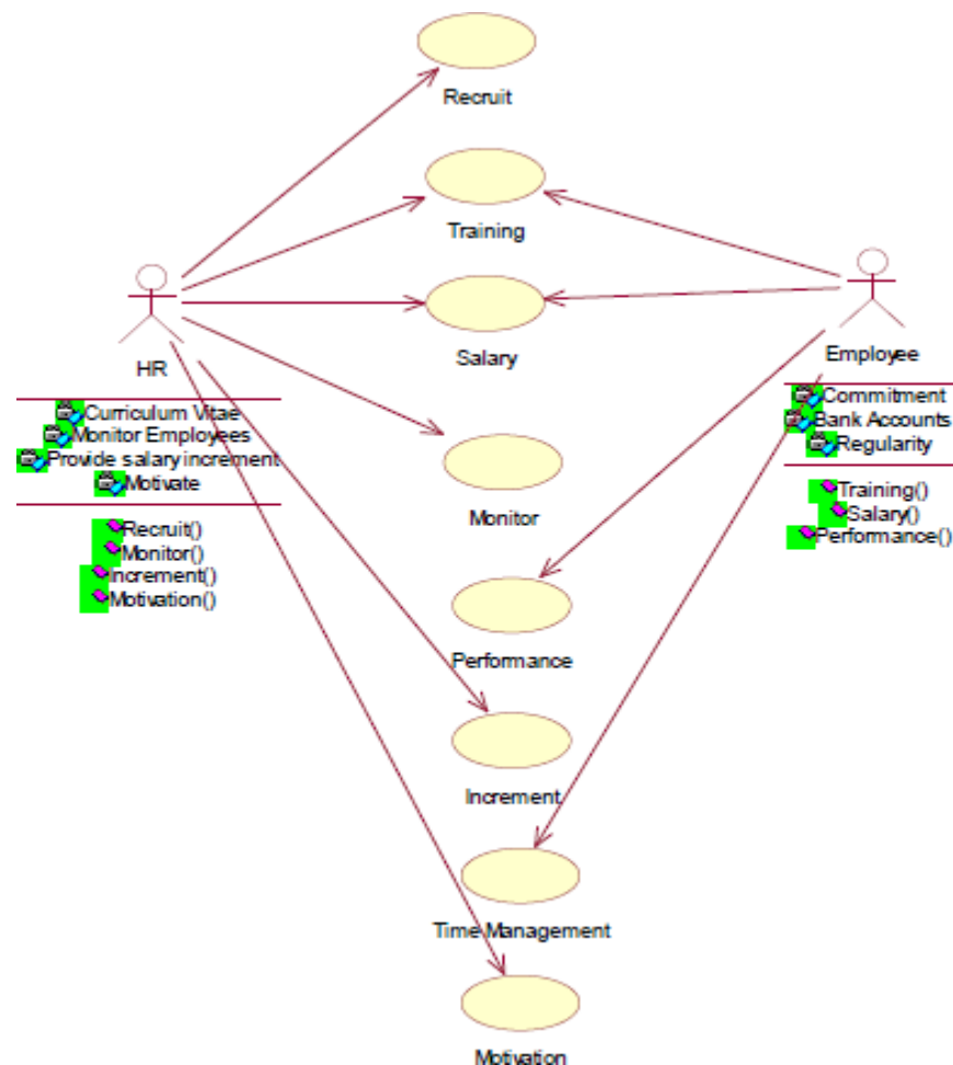
Fig.3.USE CASE DIAGRAM
