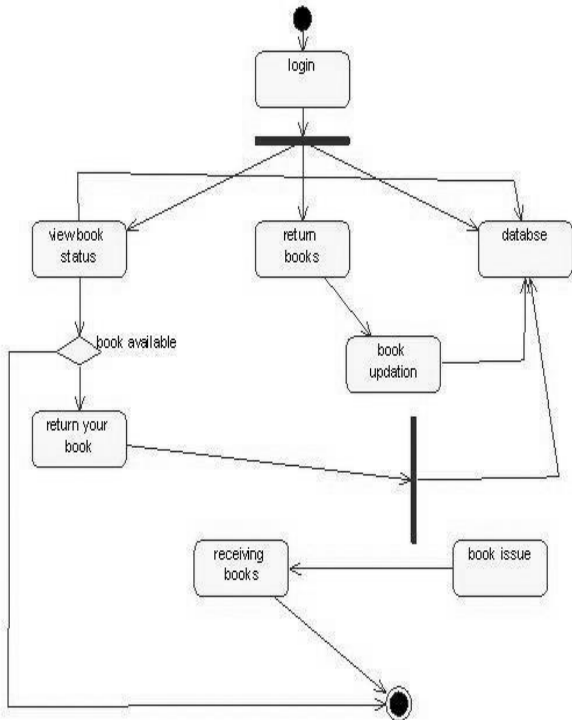
Fig.4.ACTIVITY DIAGRAM
