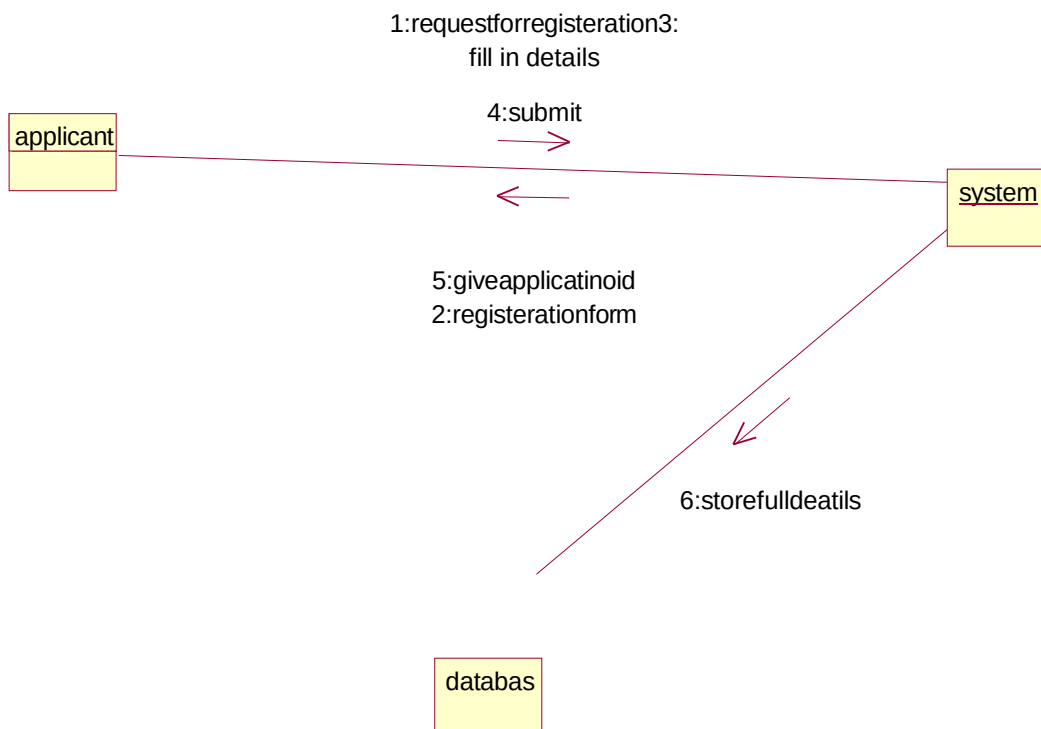
Fig.6.6.COLLABORATION DIAGRAM FOR NEW REGISTRATION
