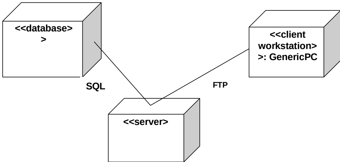
Fig.9.1.DEPLOYMENT DIAGRAM
