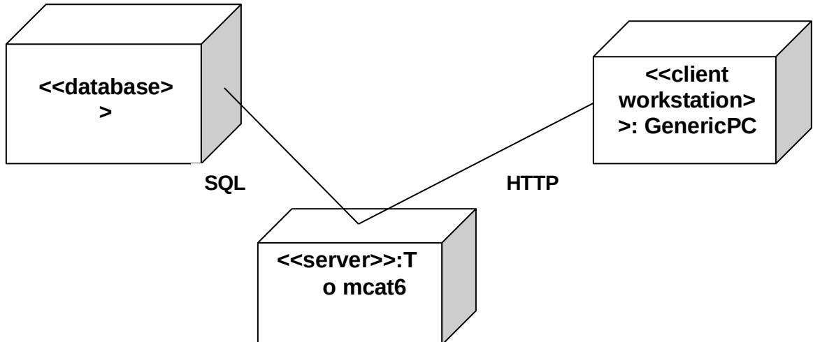
Fig.8.1.DEPLOYMENT DIAGRAM
